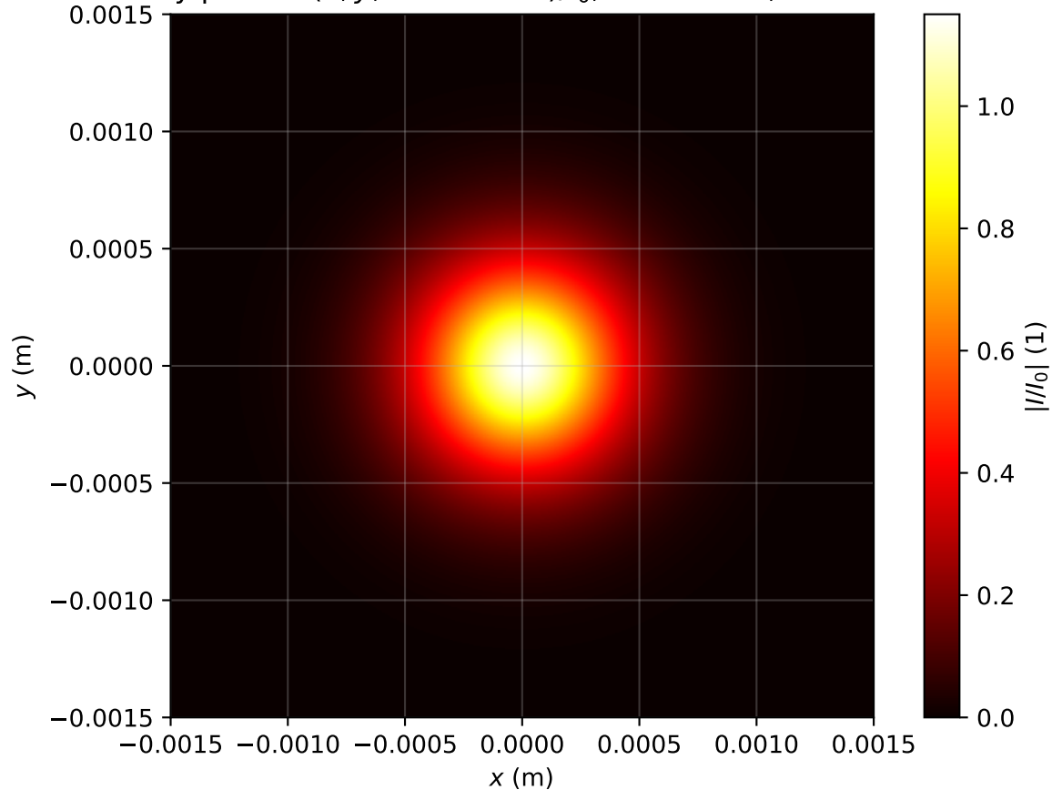
Intensity profile I(x, y, z = 0.716m)/I_0 , P_{in}=0.7P_{cr} , artificial time
